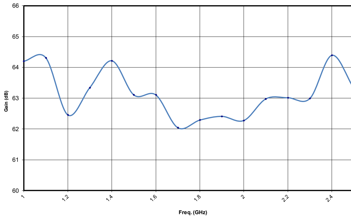
TYPICAL SMALL SIGNAL GAIN @ -20dBm INPUT
