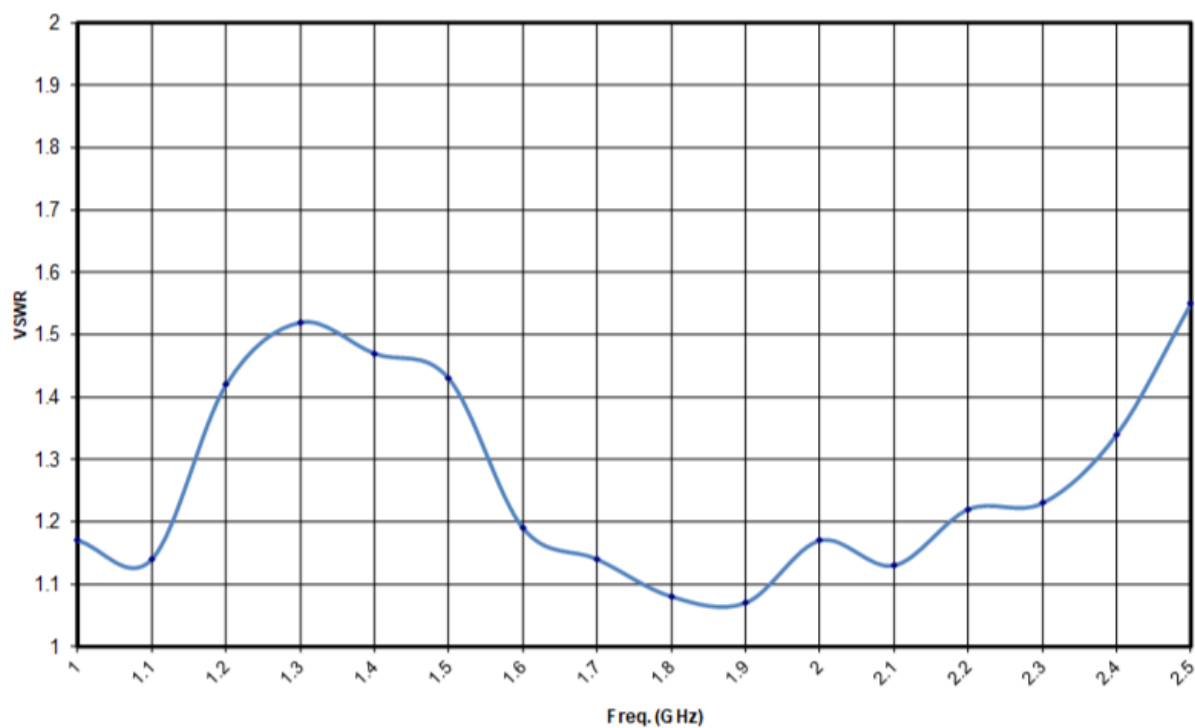
TYPICAL INPUT VSWR
