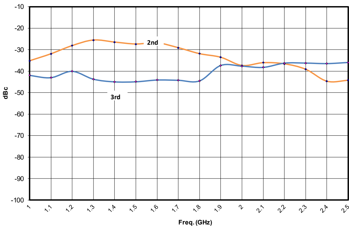
TYPICAL HARMONICS @ 350 WATTS
