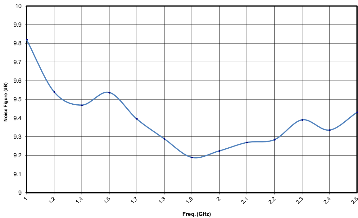
TYPICAL NOISE FIGURE
